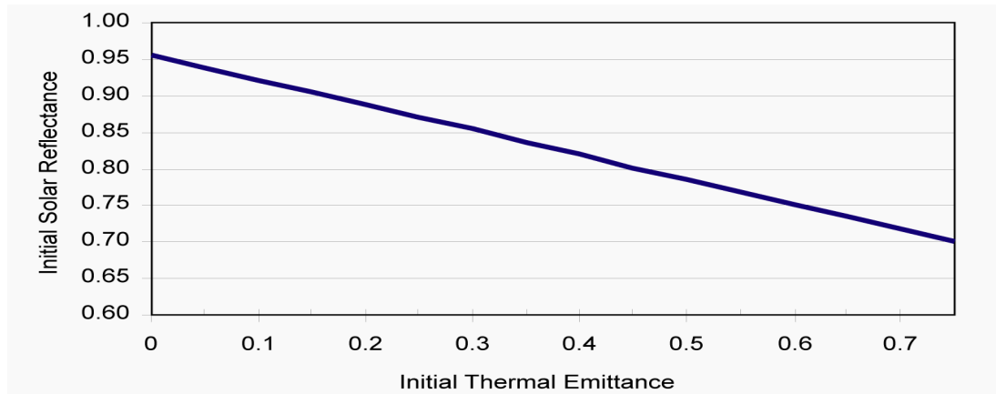
Figure 3-17 – Tradeoffs between Cool Roof Reflectance and Emittance A cool roof may comply with an emittance lower than 0.75 as long as the reflectance is higher. This graph shows the relationship.
