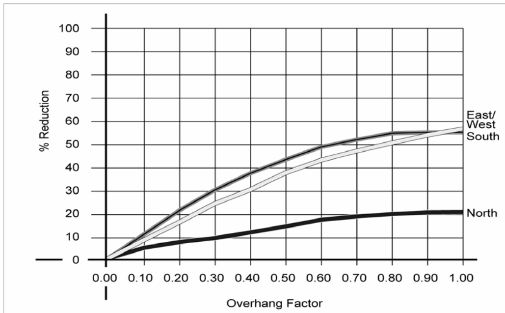
Figure 3-10 – Graph of Overhang Factors
