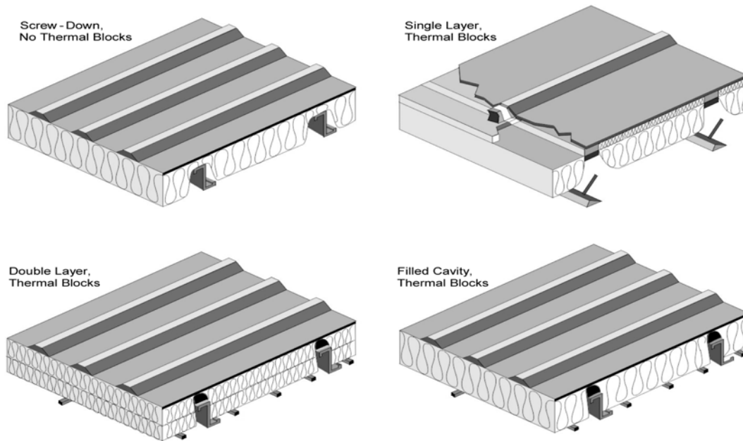
"Metal Building Roofs" Source: ACM Joint Appendix IV Table IV.7 - U-factors for Metal Building Roofs
