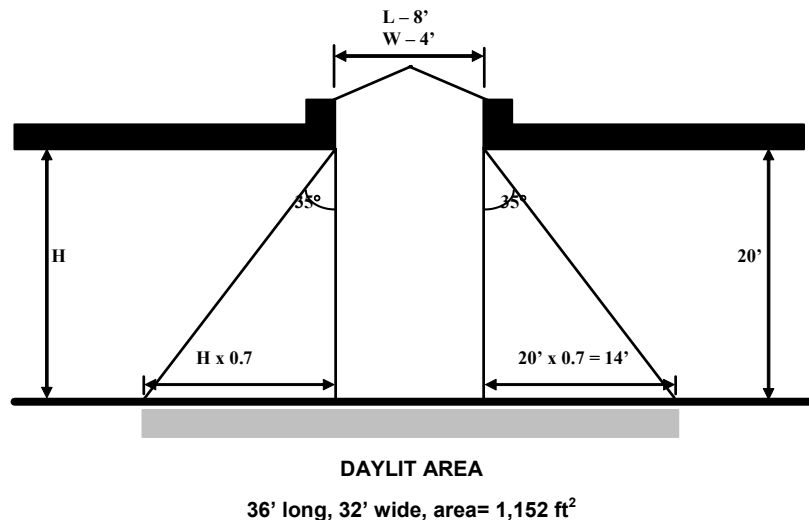
Figure 8-1 – Window Daylit Area
