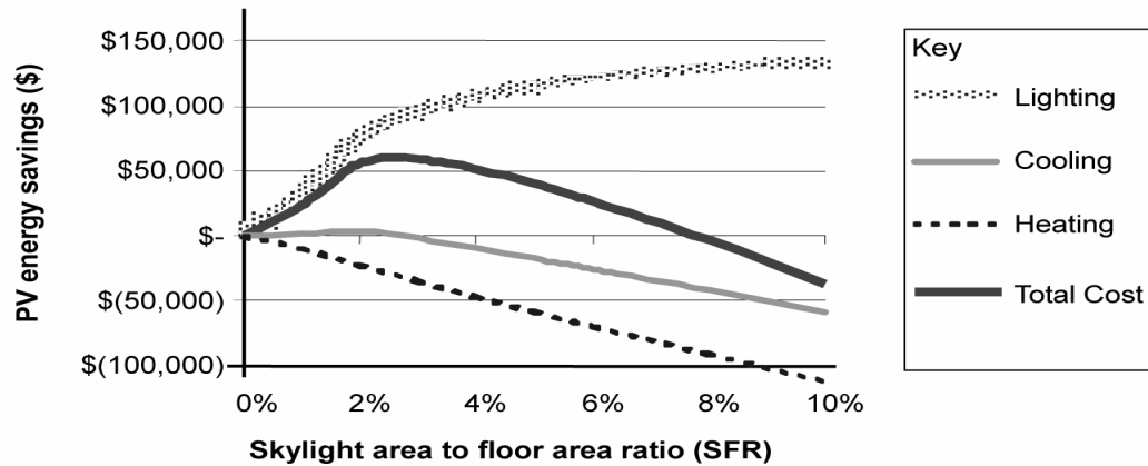
Figure 3-7 – Present Value Savings of Skylight 50,000 ft² Warehouse in Sacramento
