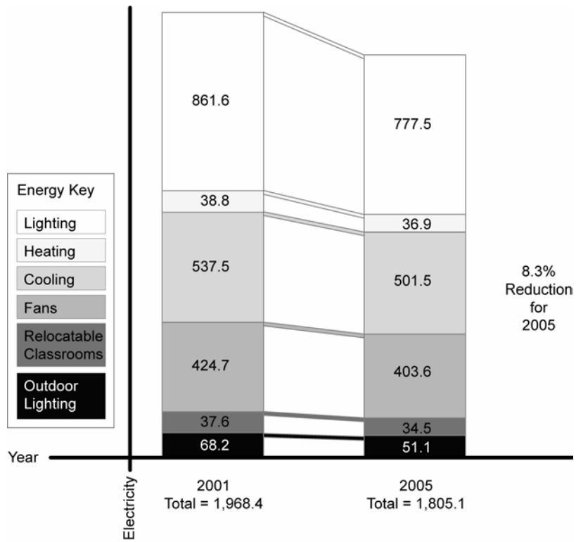
Figure 1-1 – Electricity Savings Related to the 2005 Standards
