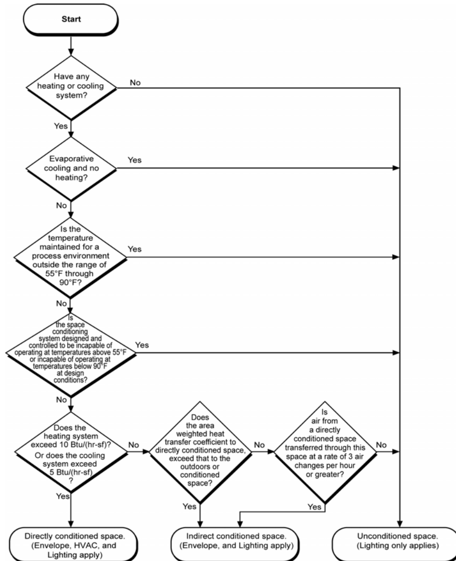
Figure 1-3 – Type of Conditioned Space and Scope of Compliance
