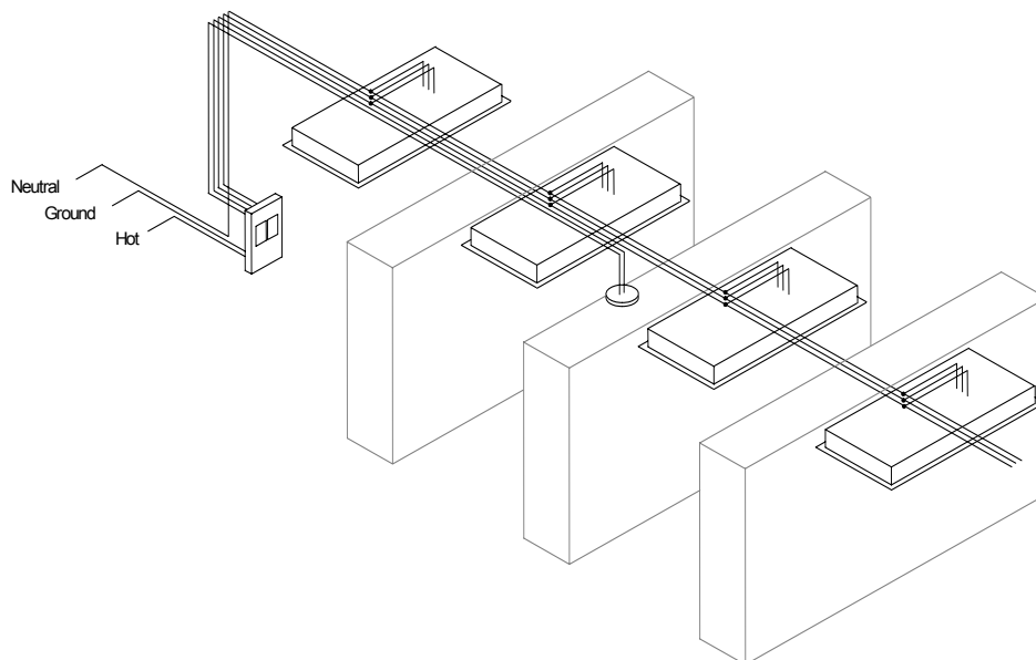
Figure 5-19 – Photocell Dimming
