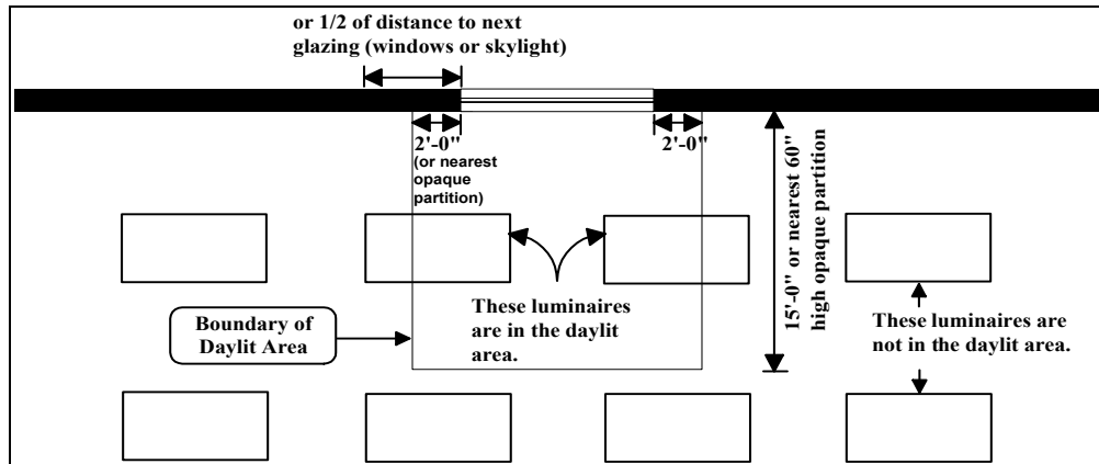
Figure 8-3 – Window Daylit Area
