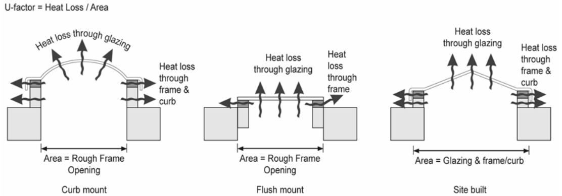
Figure 3-6 – Skylight Area
