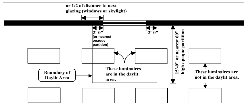
Figure 5-6 – Plan View of Daylit Area near Window
