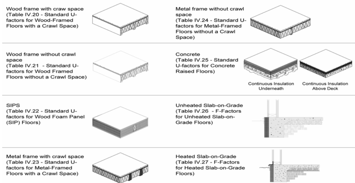
Figure 3-14 – Requirements for Floor/Soffit Surfaces
