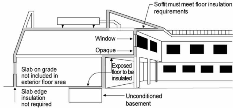
Figure 3-14 – Requirements for Floor/Soffit Surfaces
