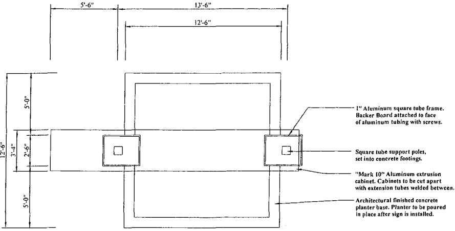
SIGN TYPE 1.0 SIGN PLAN VIEW Scale: 1/4" = 1'-0"
