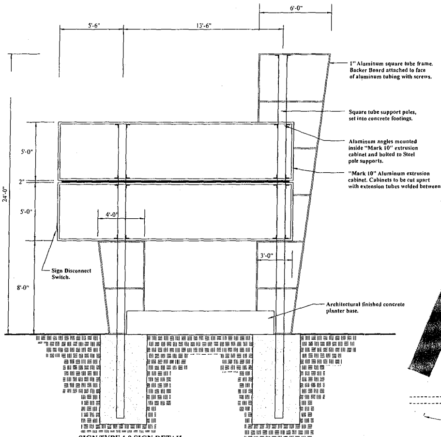
SIGN TYPE 1.0 SIGN DETAIL Scale: 1/4" = 1'-0"
