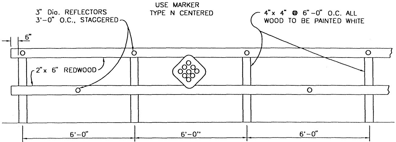
ELEVATION VIEW
